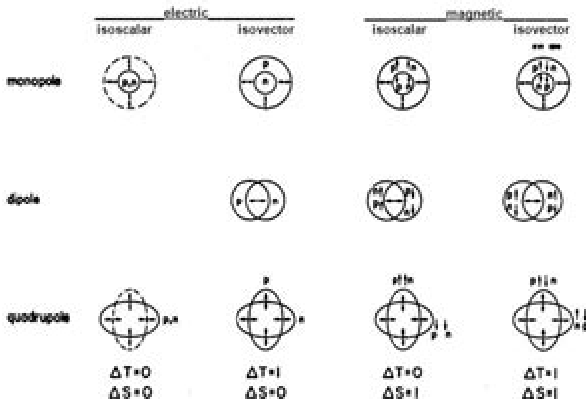
FIG. 2. Qualitative picture of giant resonance modes of the nucleus.
