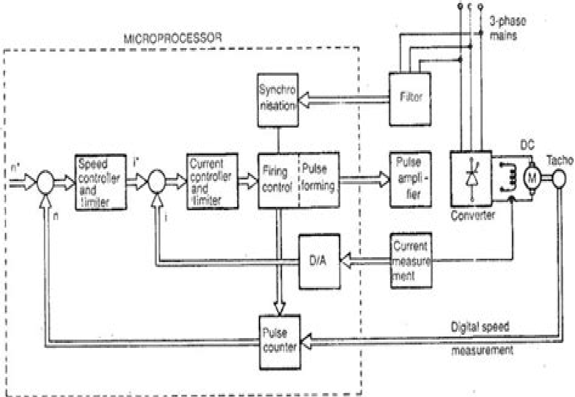
Fig. 8.6(b) Block diagram of a separately excited dc motor drive using a microprocessor
