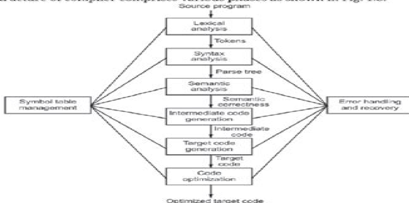
Fig. 1.8: Phases of a Compiler
