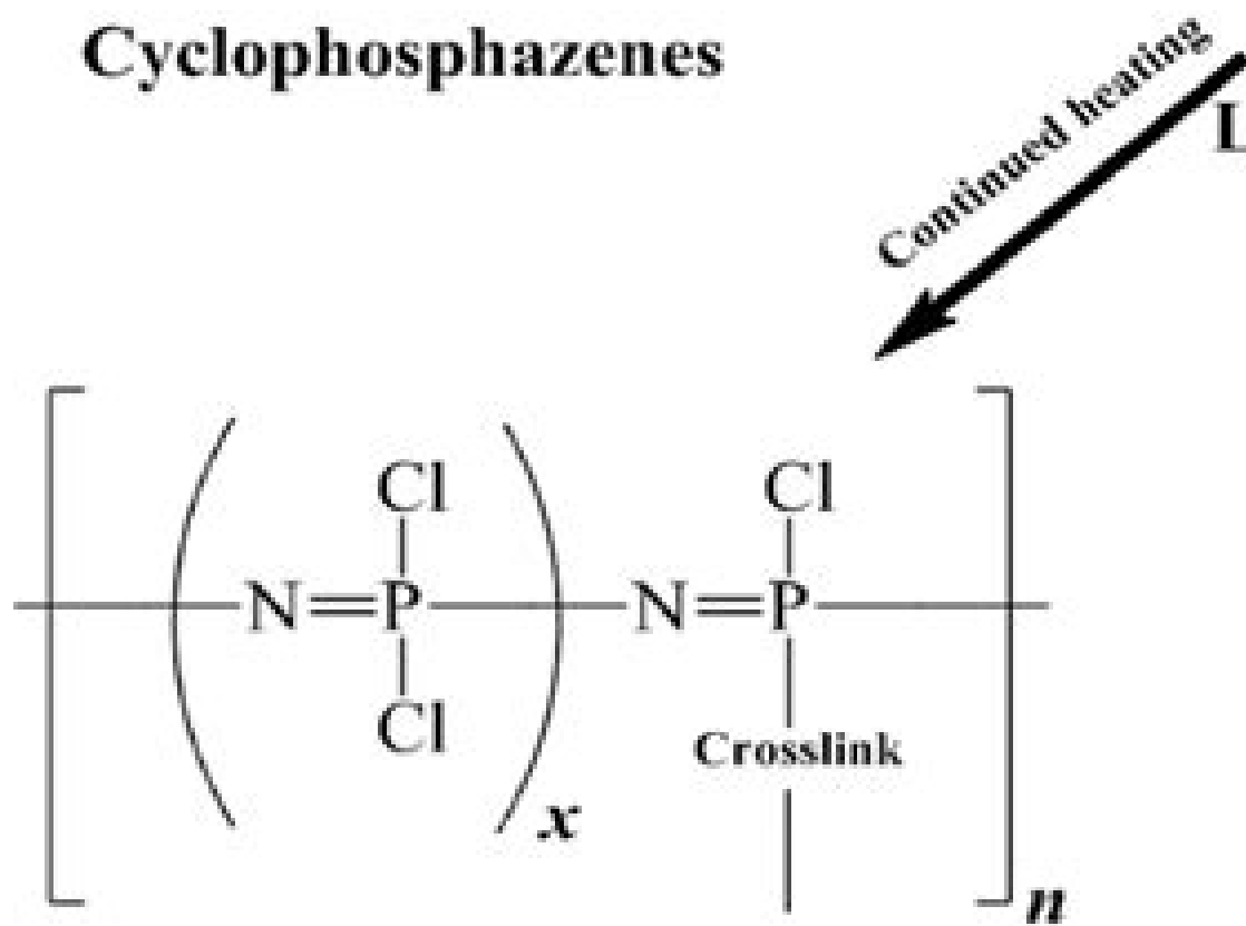
Macromolecular polyphosphazenes
