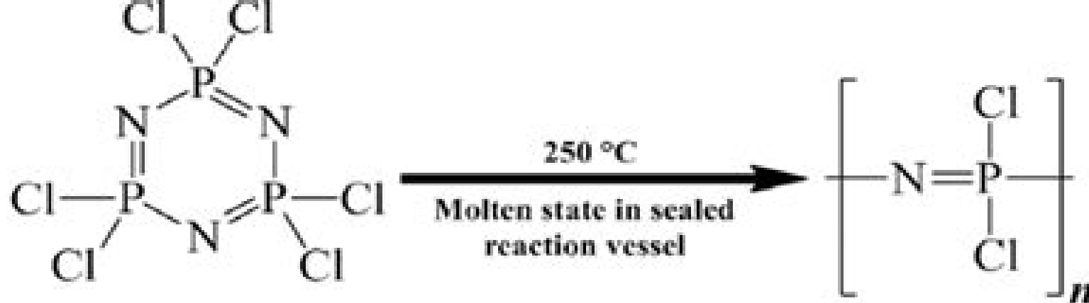
Cyclophosphazenes
