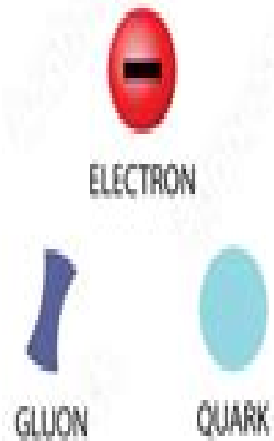
Elementary particles
