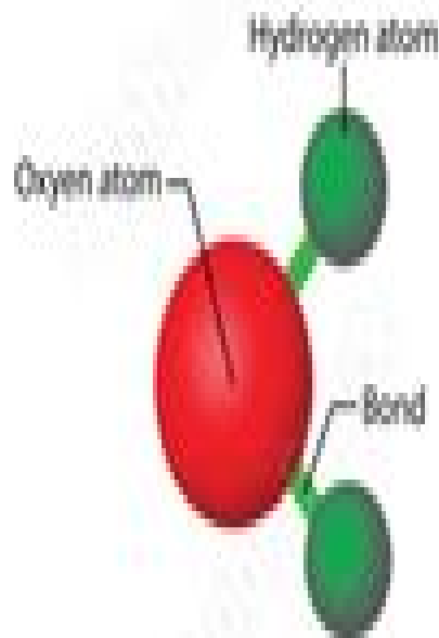
Molecule
