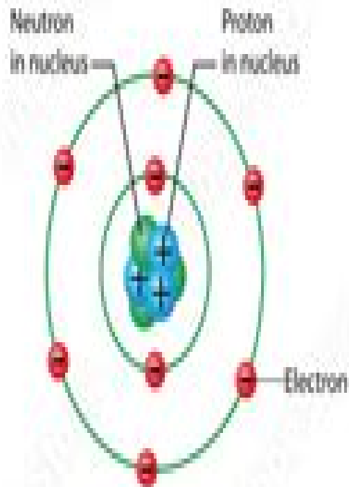
Atom
