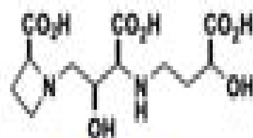
Mugineic acid
