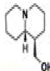
(+)-Epilupinine
