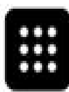
Perplexity
