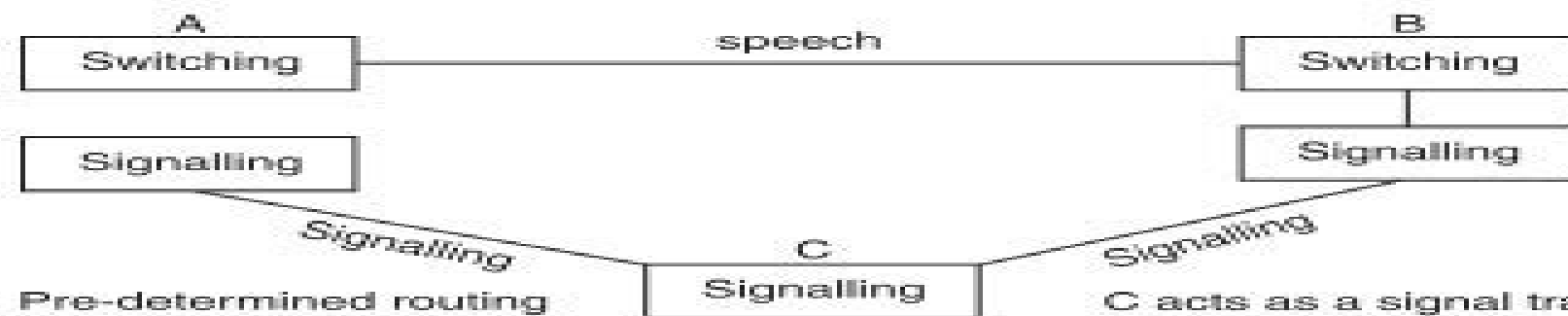
(b) Common channel signalling between A and B on a quasi-associated basis
