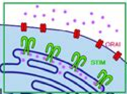
Full \text{Ca}^{2+} -store in ER-lumen
