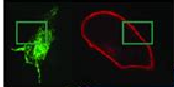
Full \text{Ca}^{2+} -store in ER-lumen
