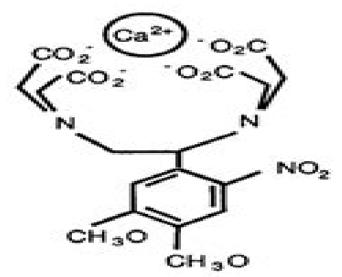
DM-nitrophen
