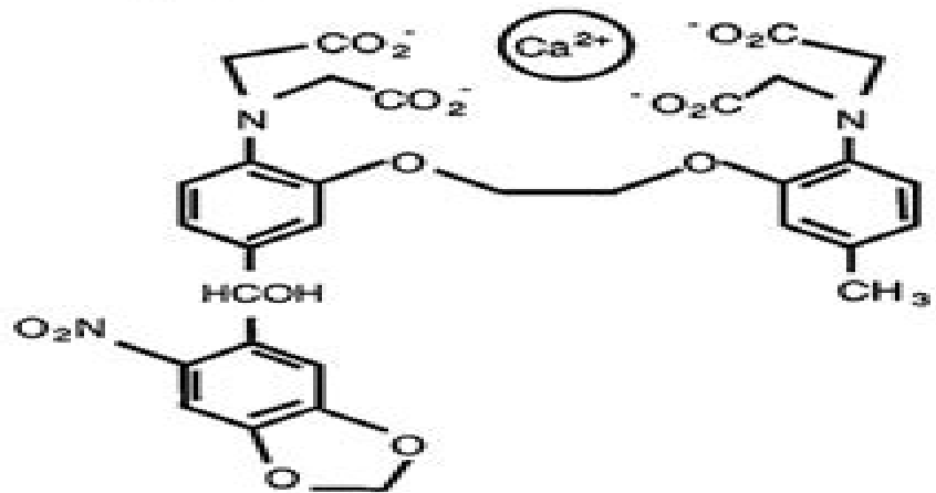
nitr-5
