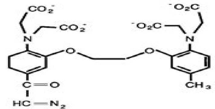
diazo-2
