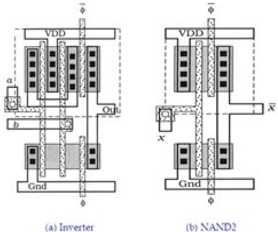
Figure 9.14 Layout examples of C 2 MOS circuits
