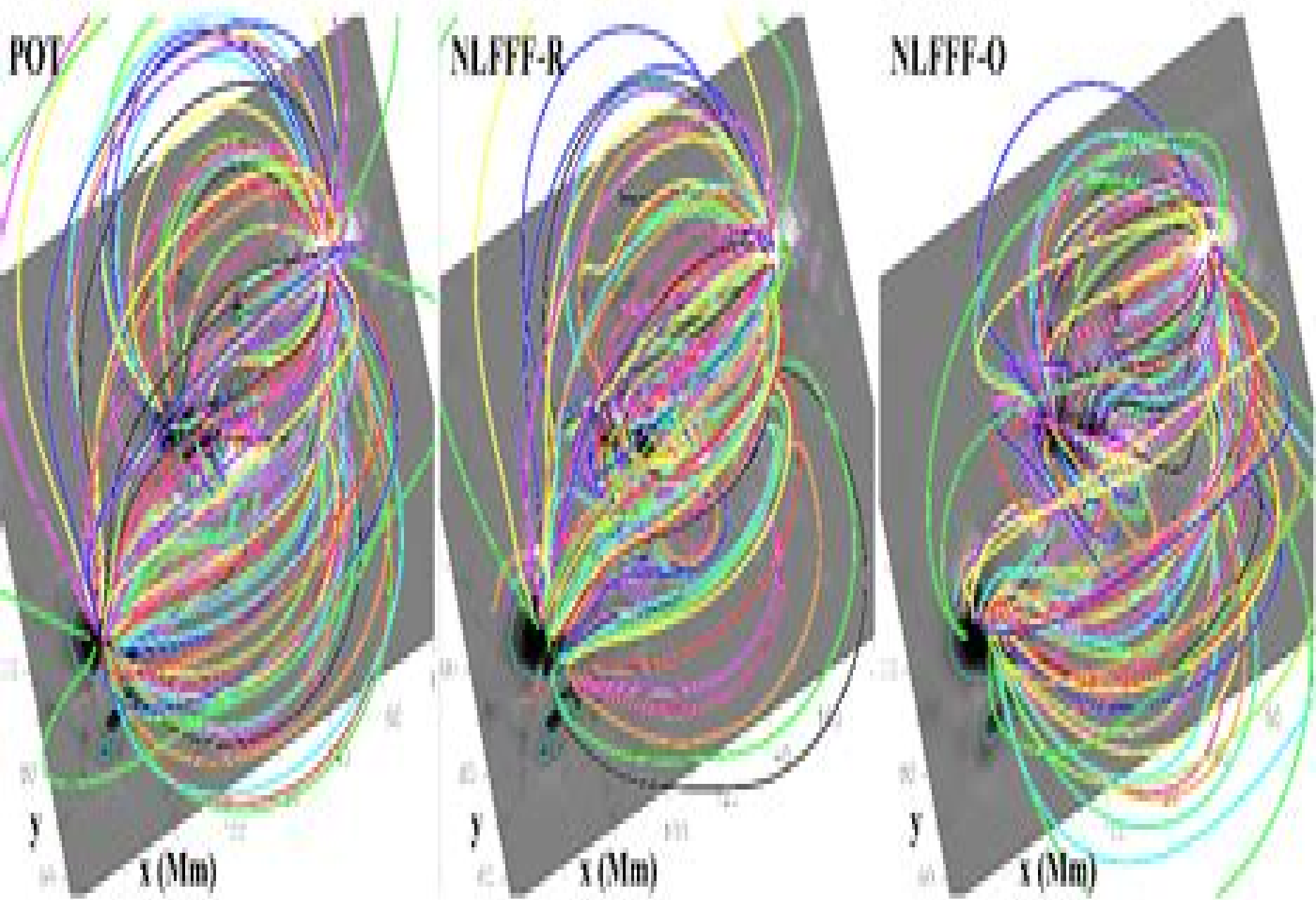
Fig. 2.— Selected closed field lines of the 3D extrapolated magnetic field for the potential field (labelled POT; left), the NLFFF from the magnetofrictional
