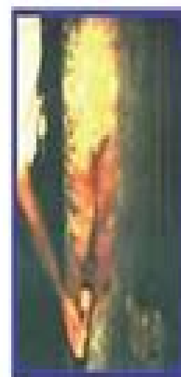
Water Intake Structure Rebar Corrosion
