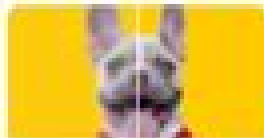
Unblur
