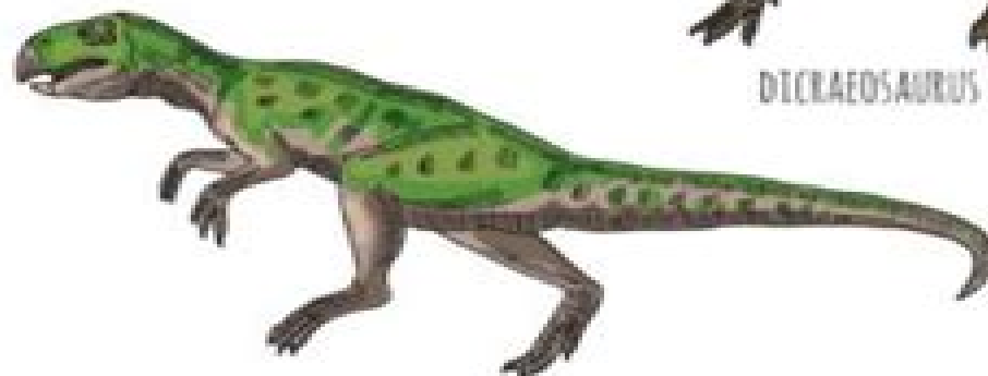
PSITTACOSAURUS
