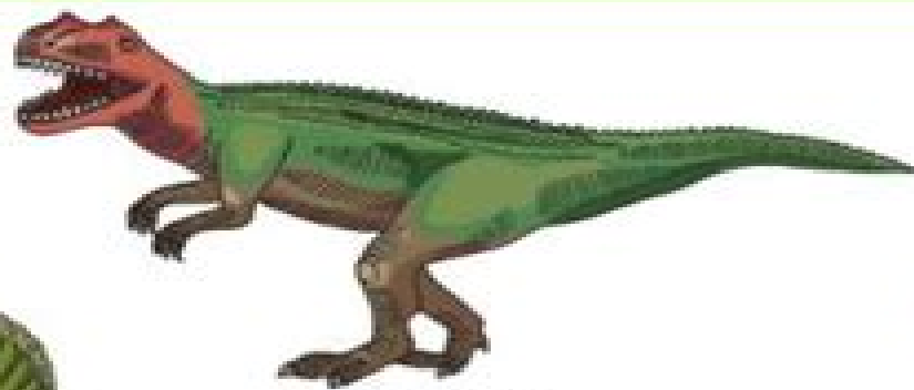
GIGANTOTYRANNUS
