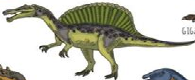
SPINOSAURUS
