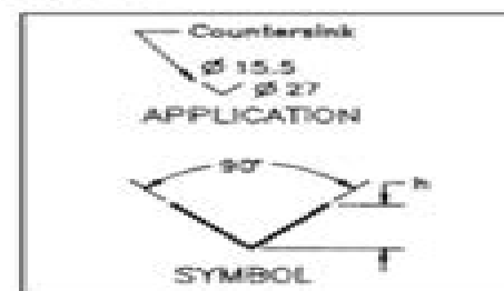
Figure 4. Countersink Symbol
