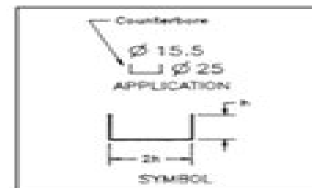
Figure 3. Counterbore Symbol
