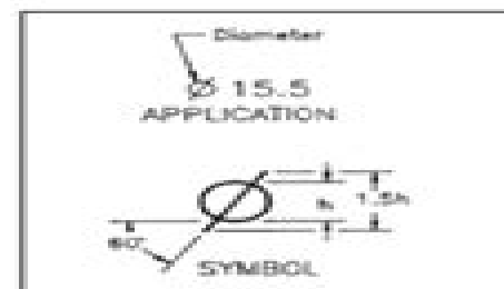
Figure 2. Diameter Symbol
