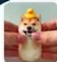
Squish
