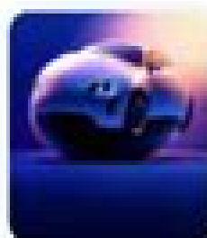
Expansion
