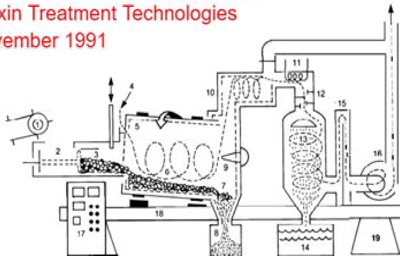
Figure 2-1—Rotary Kiln
