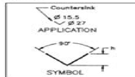
Figure 4. Countersink Symbol
