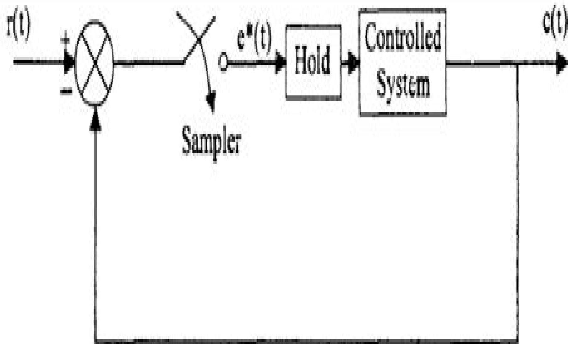
Discrete data control system
