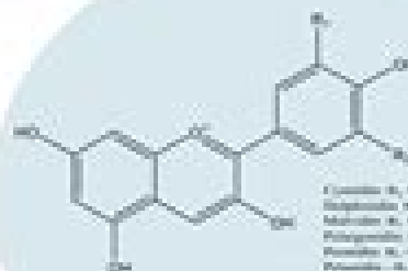
Anthocyanin
