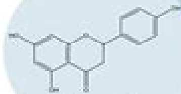
Naringenin
