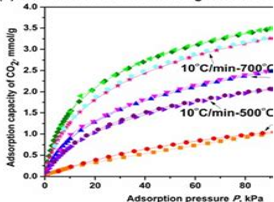
(d) activation at different heating rates and a
