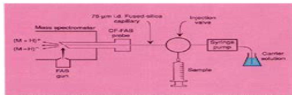
Figure 1. Instrumental arrangement for CF-FAB MS operated in the flow injection mode.
