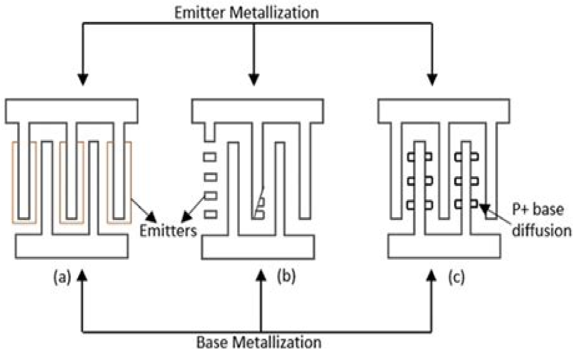
Surface geometry of n-p-n microwave transistor (a) Inter-digitated (b) Overlay (c) Matrix
