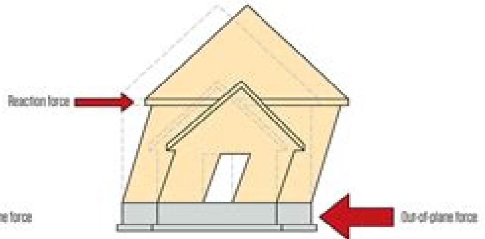
Racking
