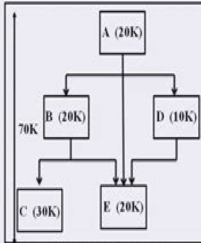
Fig: Subroutine calls between the procedure[3]
