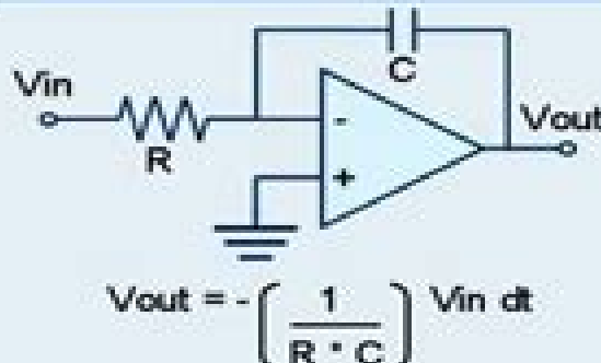
Integrator Amplifier
