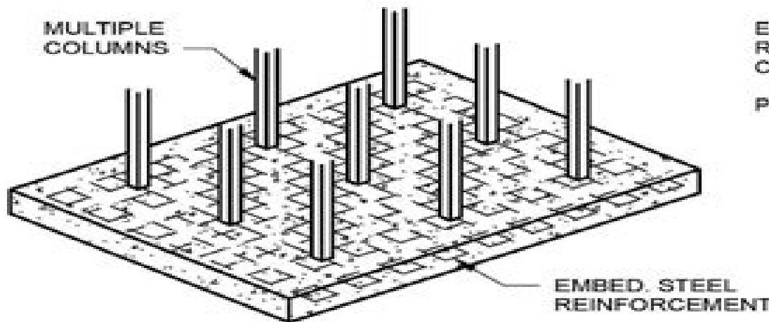
CONCRETE RAFT OR MAT FOOTING (SHALLOW FOUNDATION)
