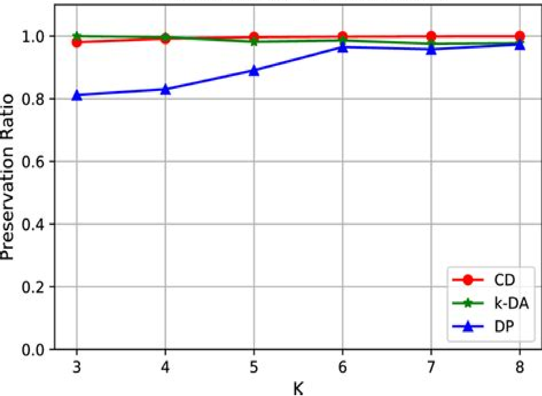
Enron: CD, k-DA, DP on Page Rank
