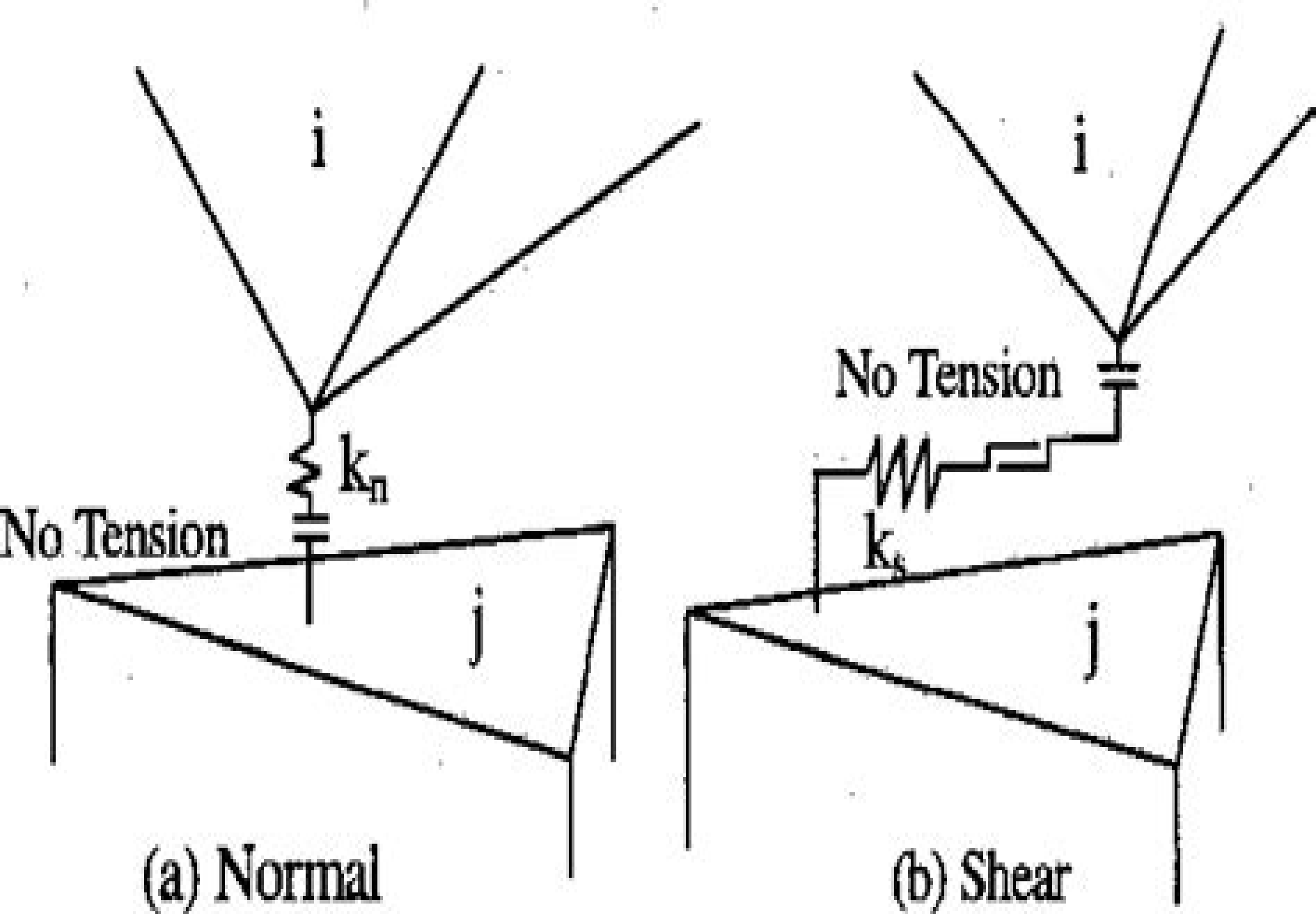
Fig. 9 Illustration of 2D DDA contact mechanisms
