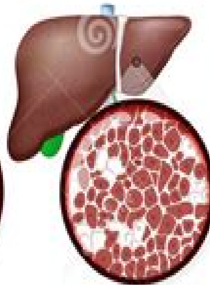
FIBROSIS
