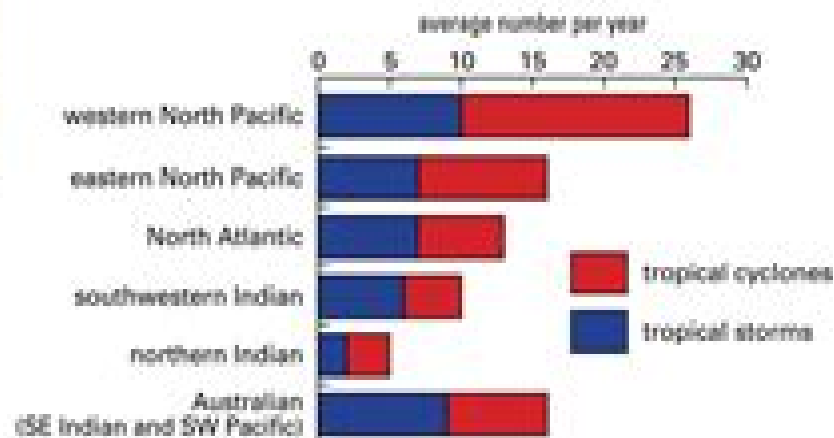
Frequency of tropical storms and tropical cyclones
