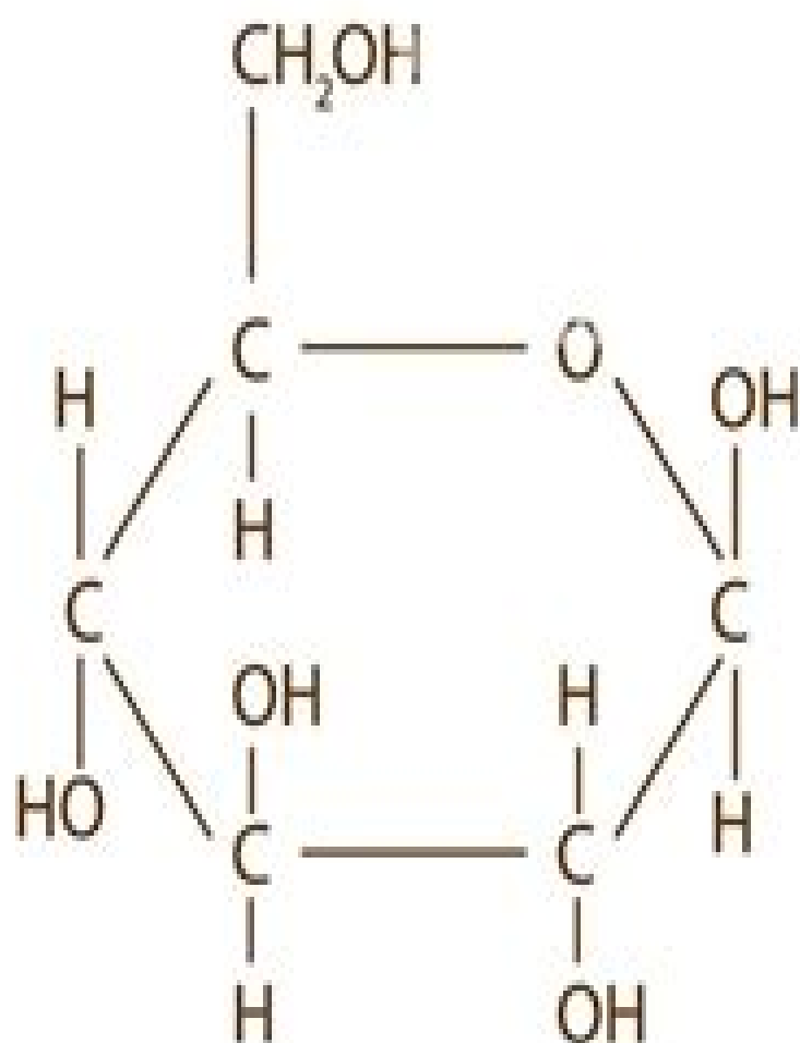
\beta -D-Glucose
