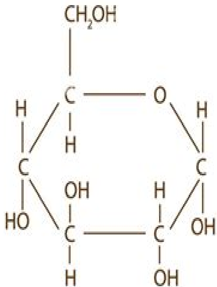
\alpha -D-Glucose
