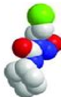
Guest molecule
