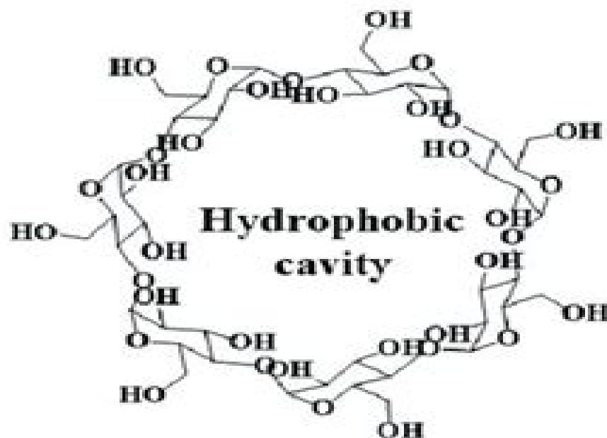
β-CD
