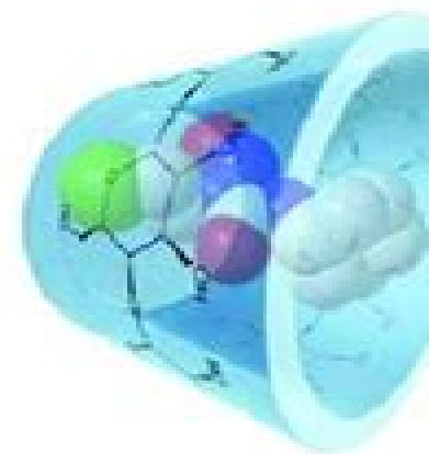
Inclusion complex
