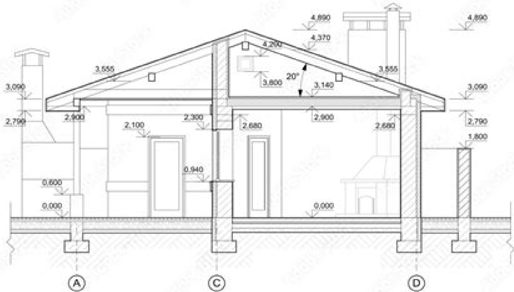
Cross section 1-1
