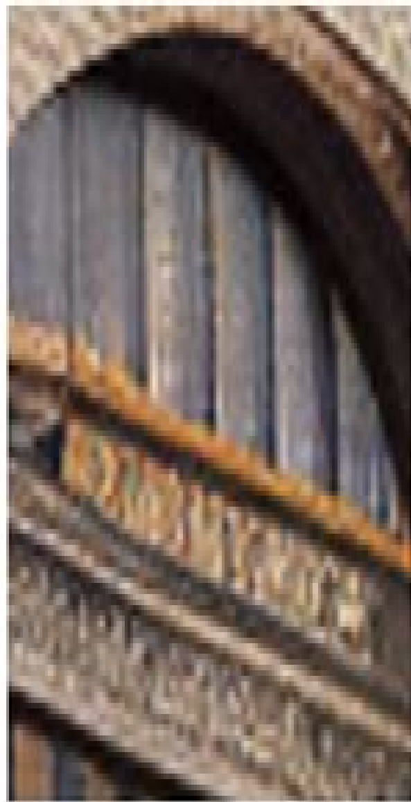
Original
