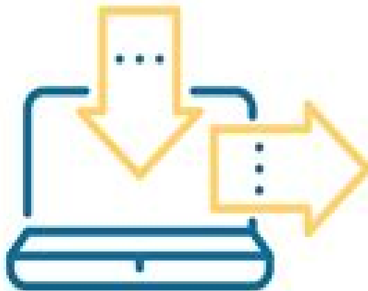
Conditional Statements
