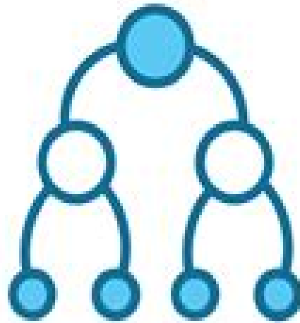
Conditional Statements
