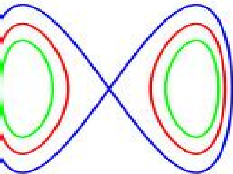
(c) "Figure eight-loop"
