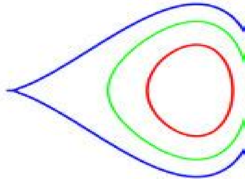
(b) "Cuspidal loop"
