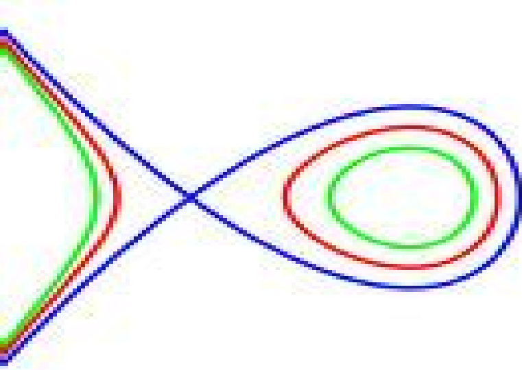
(a) "Saddle loop"
