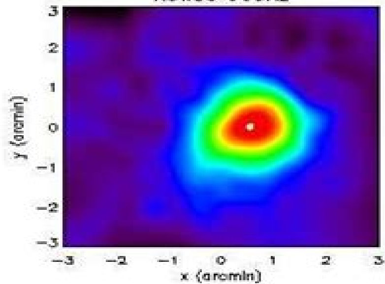
RCW38 90GHz
