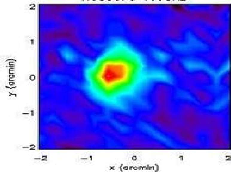
NGC3576 150GHz
