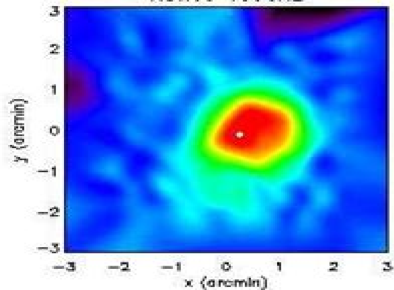
RCW38 150GHz
