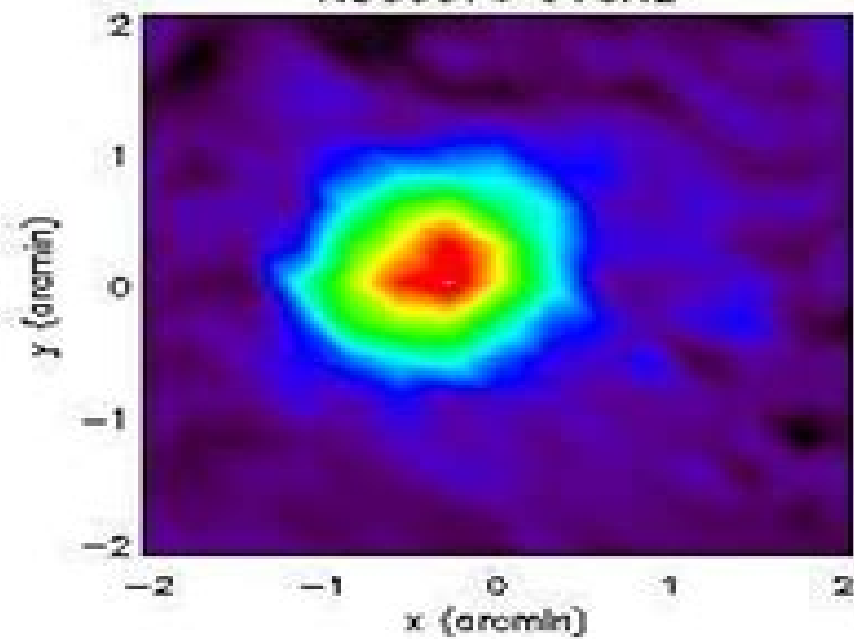
NGC3576 90GHz
