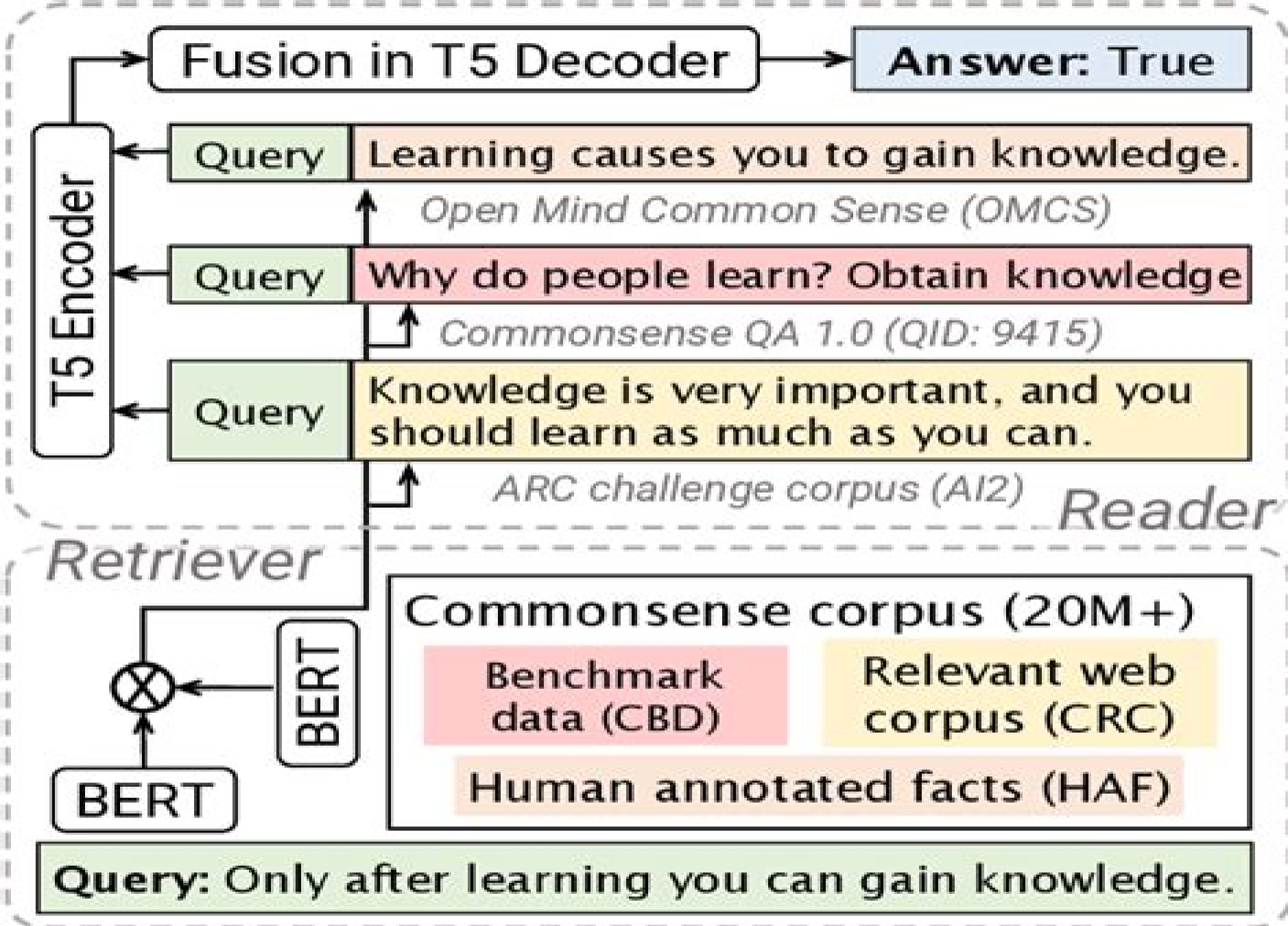
Figure 1: RACo has two major components: (i) a Retriever that takes a query and returns relevant information from a commonsense corpus, and (ii) a Reader that takes the retrieved information and the query and returns the final answer.
