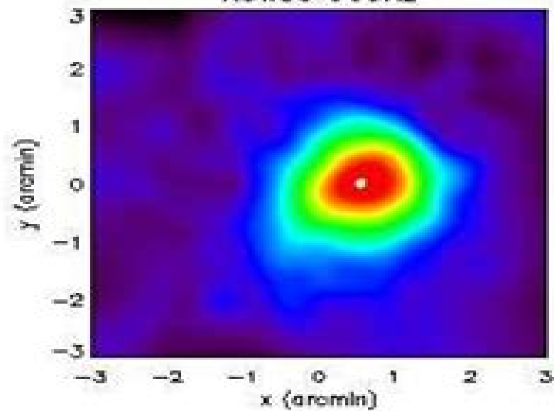
RCW38 90GHz
