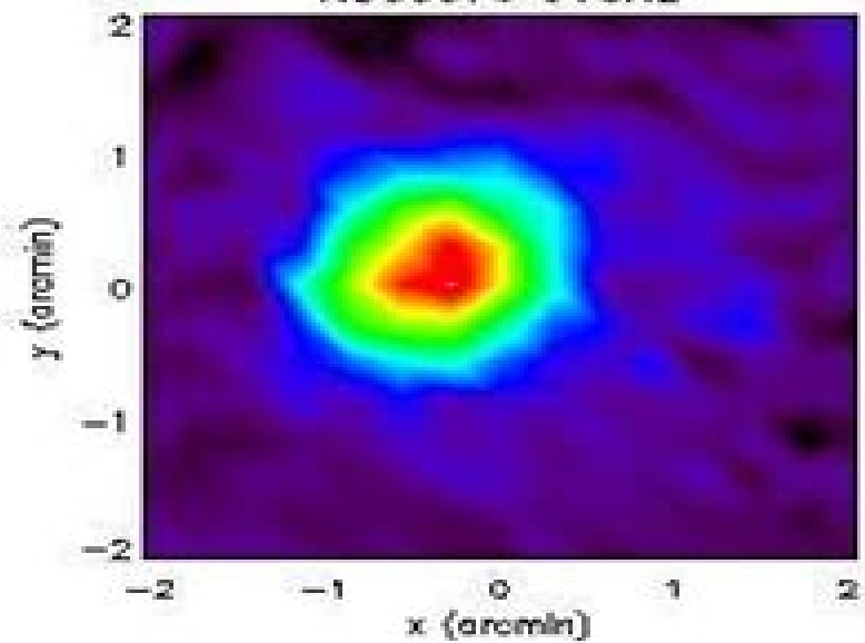
NGC3576 90GHz
