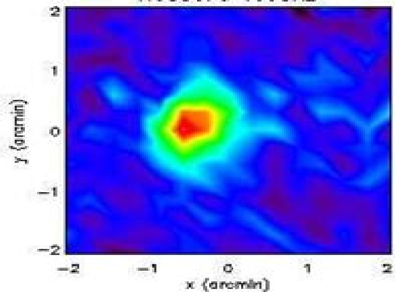
NGC3576 150GHz
