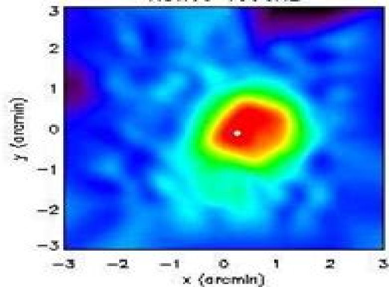
RCW38 150GHz
