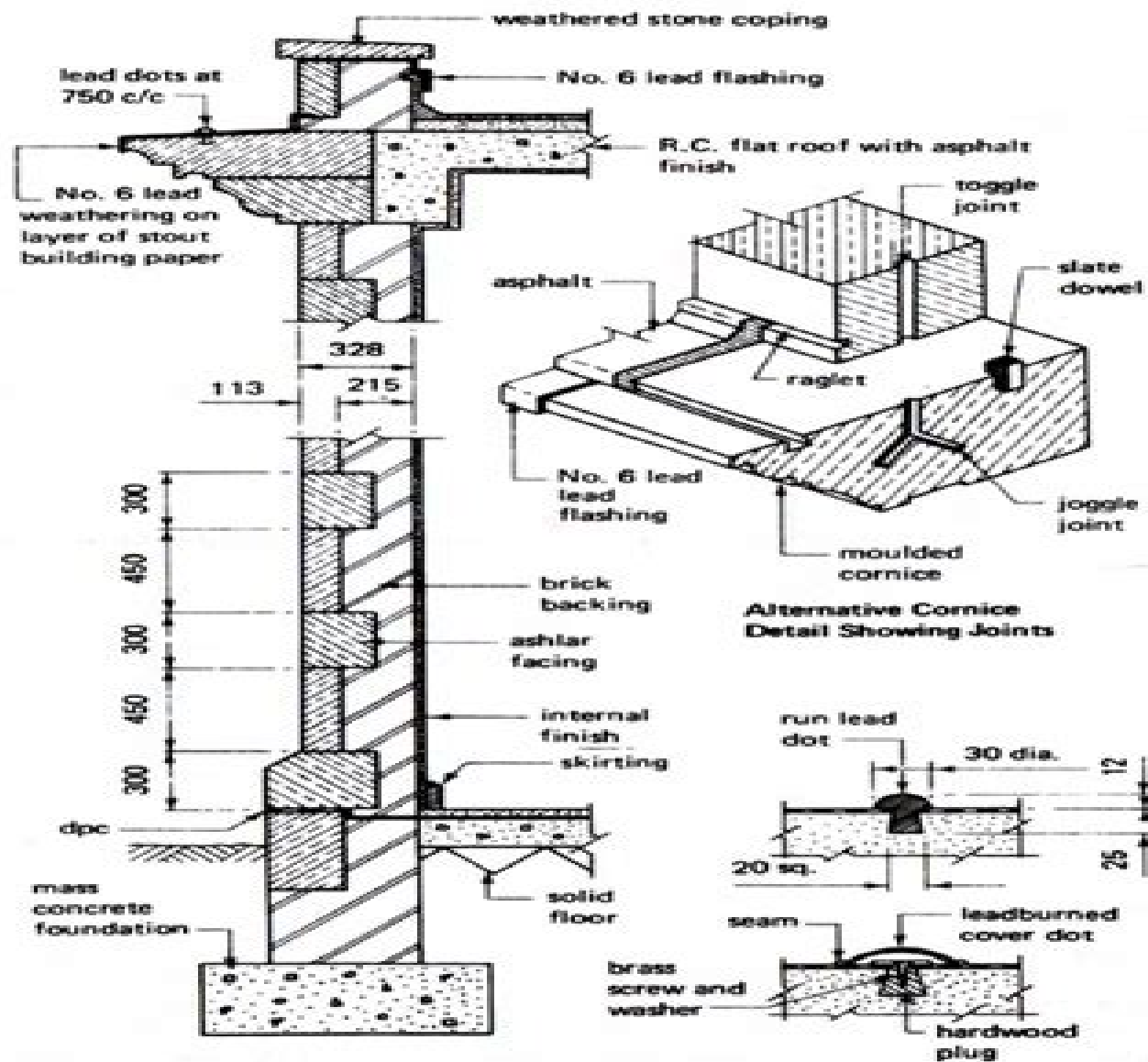
Fig. II.2 Typical details of ashlar stonework
