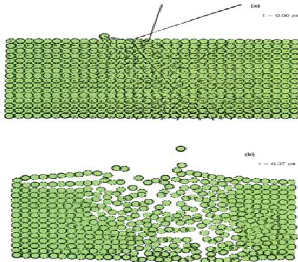
Figure 1. Two-dimensional molecular dynamics calculation (a) of the sputtering of solid KCl by 1.33 keV Ar + incident at 20° to the surface at t = 0 s. (a). Note the eventual upward movement of some particles from the initial crater and the commencement of surface peeling away from the impact site after 0.37 ps (b).
