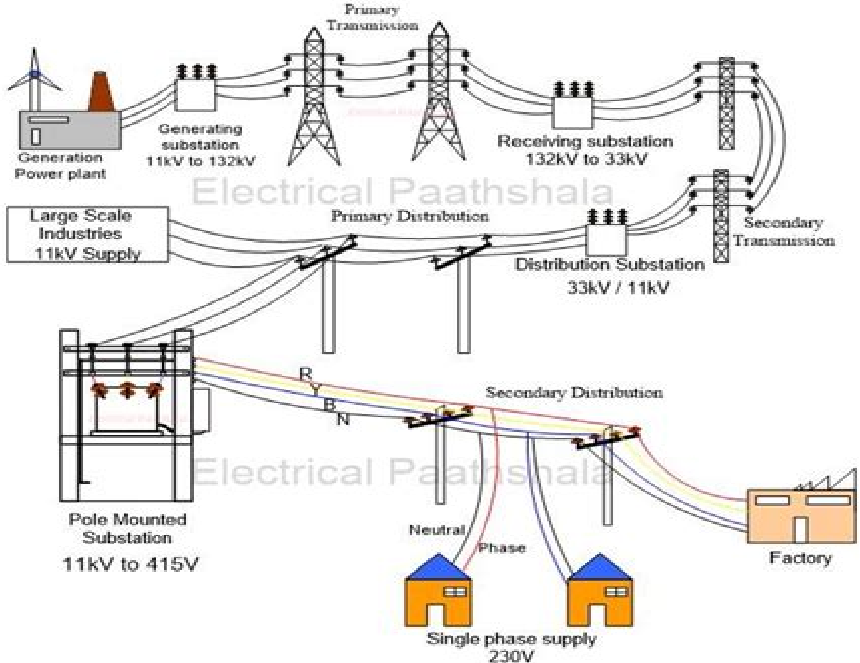
Fig. Generation, Transmission and Distribution of AC Electrical Power
