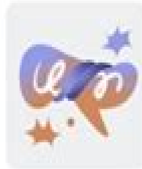
Translator
